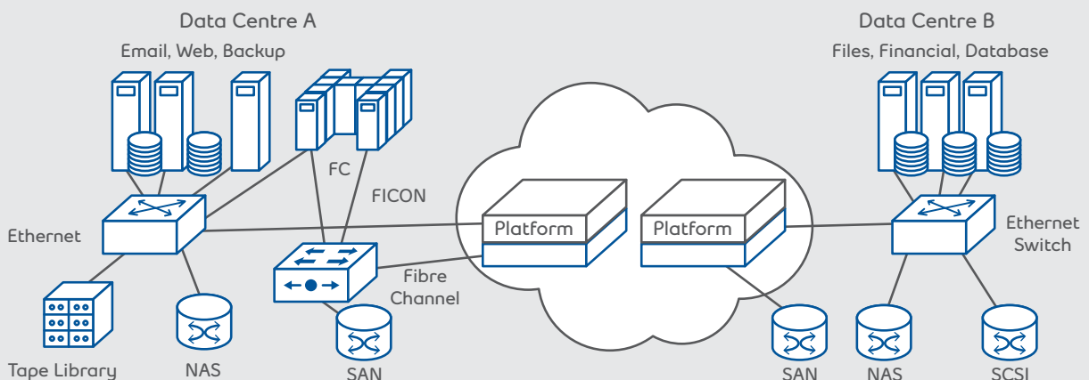
Figure 2. Interconnecting storage application between remote data centres
